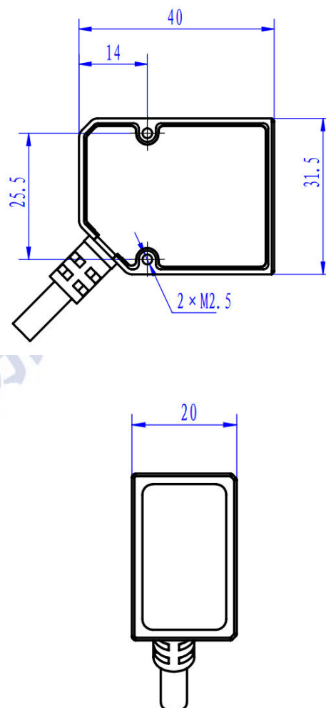
Dimensional Drawing
