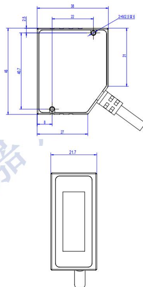
Dimensional Drawing
